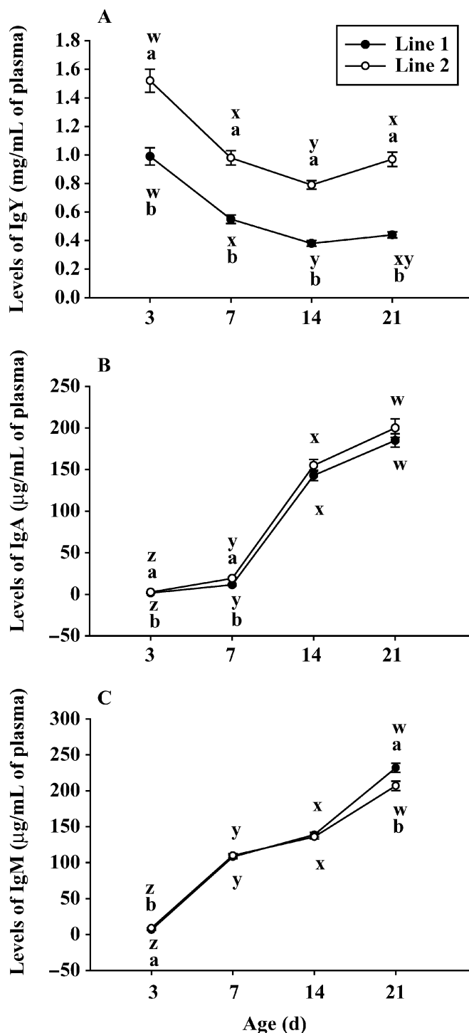
Figure 1. Plasma levels of IgY (A), IgA (B), and IgM (C) in 3-, 7-, 14- and 21-d-old chicks from 2 meat lines of chickens. The chicks were hatched from consecutively laid fertile eggs collected when the hens were 39 wk of age. The hens were vaccinated for bacterial and viral poultry pathogens following standard vaccination protocol used by the breeding company. The chicks (4 to 5/dam; line 1, 17 hens; line 2, 21 hens) were raised on wood shavings litter in a HEPA-filtered isolation room. The chicks were not vaccinated, and no medication was given during the 21-d study period. Plasma levels of IgY, IgA, and IgM were determined using chicken IgY, IgA, and IgM quantitative ELISA kits. There was no line \times time interaction for IgY ( P = 0.69 ) and IgM ( P = 0.13 ), but there was significant line \times time interaction for IgA ( P = 0.01 ). For each time point, antibody levels are expressed as means \pm SEM, and the means are based on 72 chicks from line 1 and 72 chicks from line 2. Letters a and b indicate line differences and letters w, x, y, and z indicate differences among the different time points within a line; for each analysis, means without a common letter are different ( P \leq 0.05 ).
